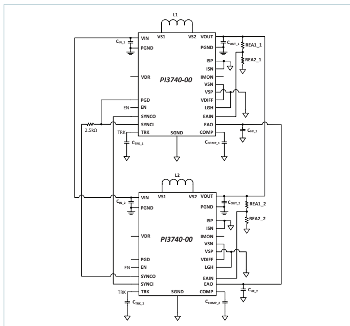
Figure 58 — PI3740-00 parallel operation
