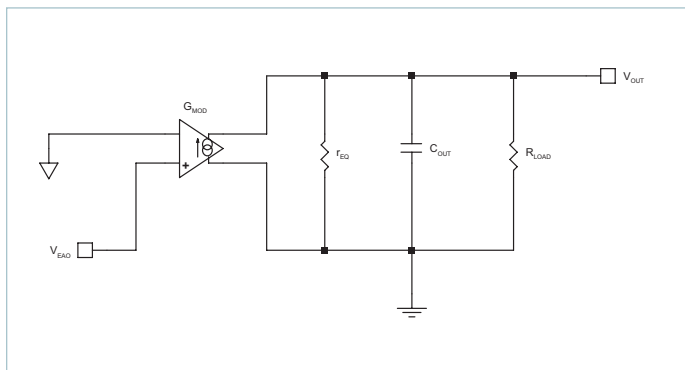
Figure 59 — PI3740-00 small-signal model control-output
