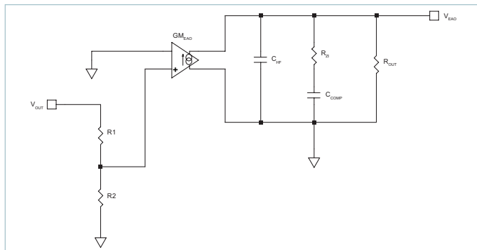
Figure 60 — PI3740-00 error amplifier model
