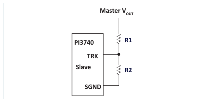
Figure 39 — Voltage divider connections for direct tracking
