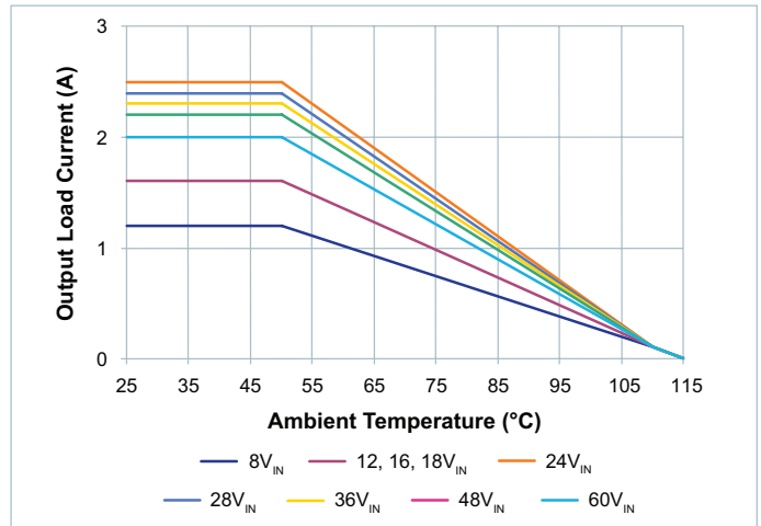
Figure 57 — Thermal de-rating for PI3740-00 evaluation board at V_{OUT} = 50V, OLFM
