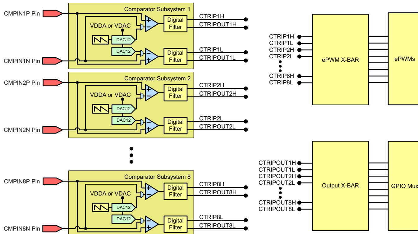
图 5-34. CMPSS Connectivity (337-Ball ZWT and 176-Pin PTP)
