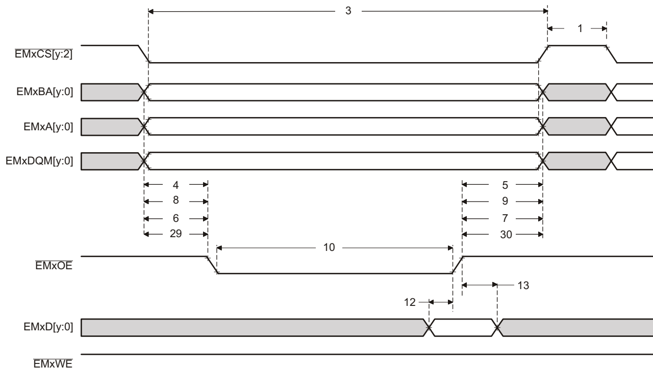
Figure 5-20. Asynchronous Memory Read Timing
