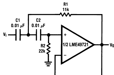
Figure 77. Sine Wave Oscillator
