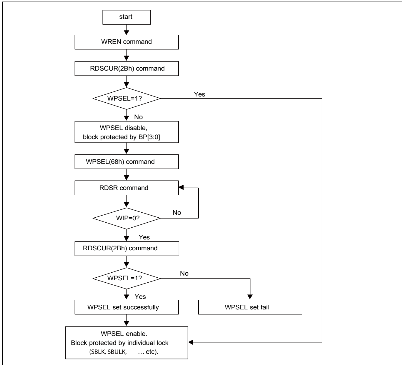
Figure 52. WPSEL Flow
