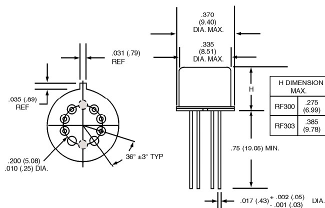
EXTERNAL DIMENSIONS
