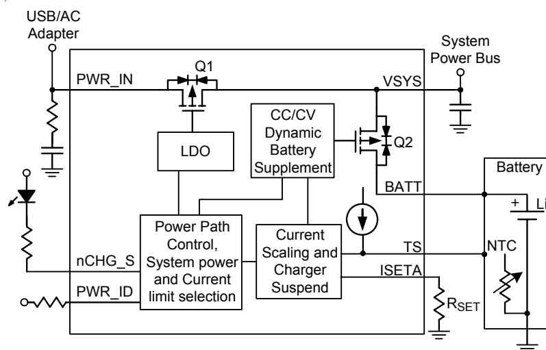
Figure 12. Charger Block Diagram and Required External Components
