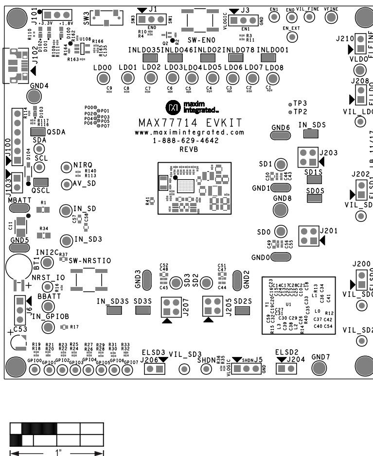
MAX77714 EV Kit Component Placement Guide—Top Silkscreen
