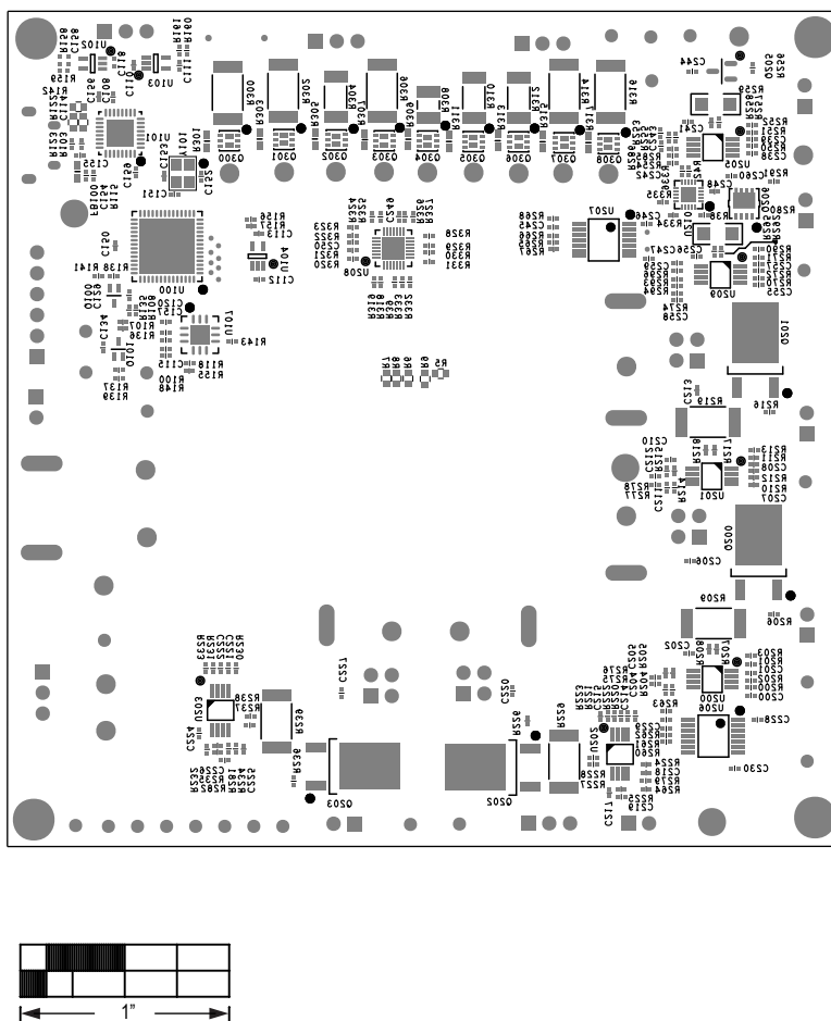
MAX77714 EV Kit Component Placement Guide—Bottom Silkscreen
