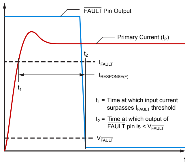
Figure 3: Overcurrent Fault Response
