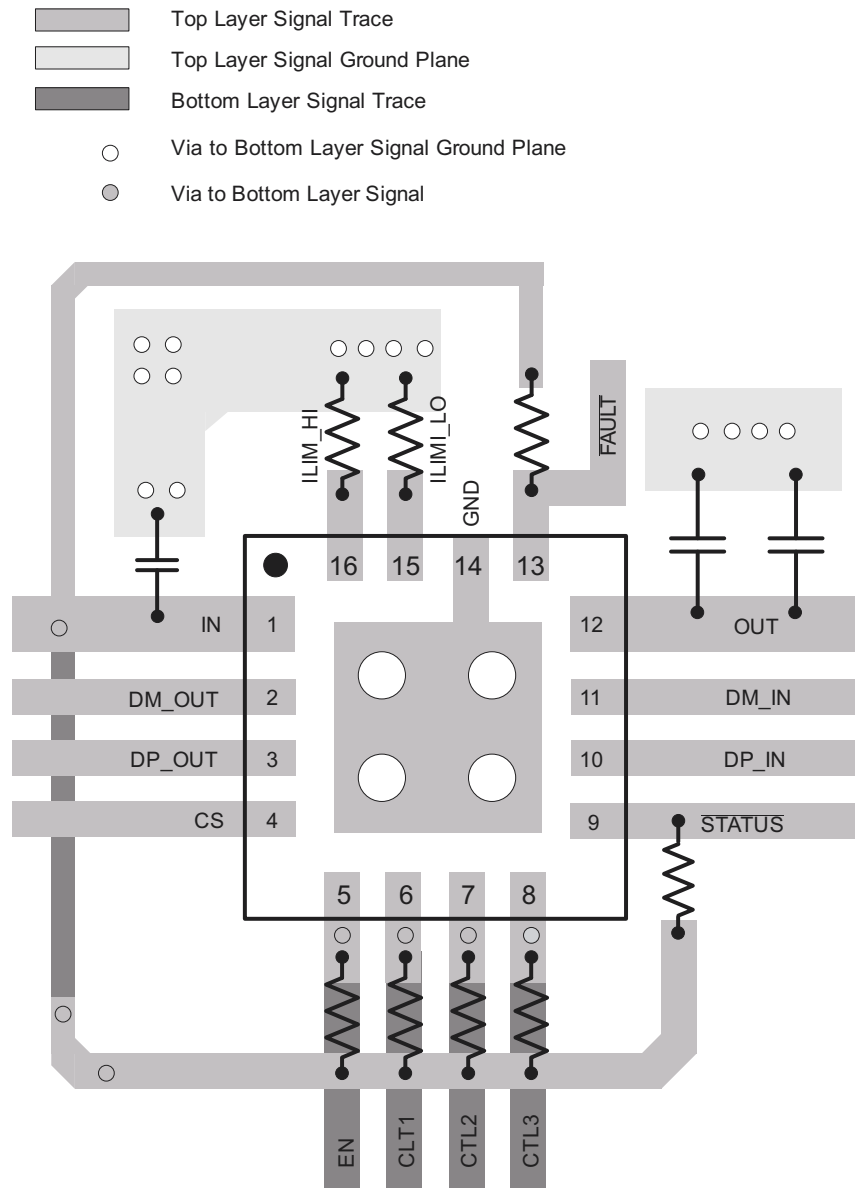
Figure 58. TPS2549-Q1 Layout Diagram
