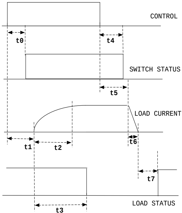
Figure 2 - Timing Diagram
