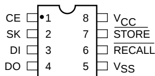
DIP Package (P, L, GL)
