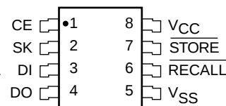
SOIC Package (S, V, GV)
