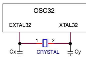
Figure 36. RTC Oscillator (OSC32) module connection – Diagram 1
