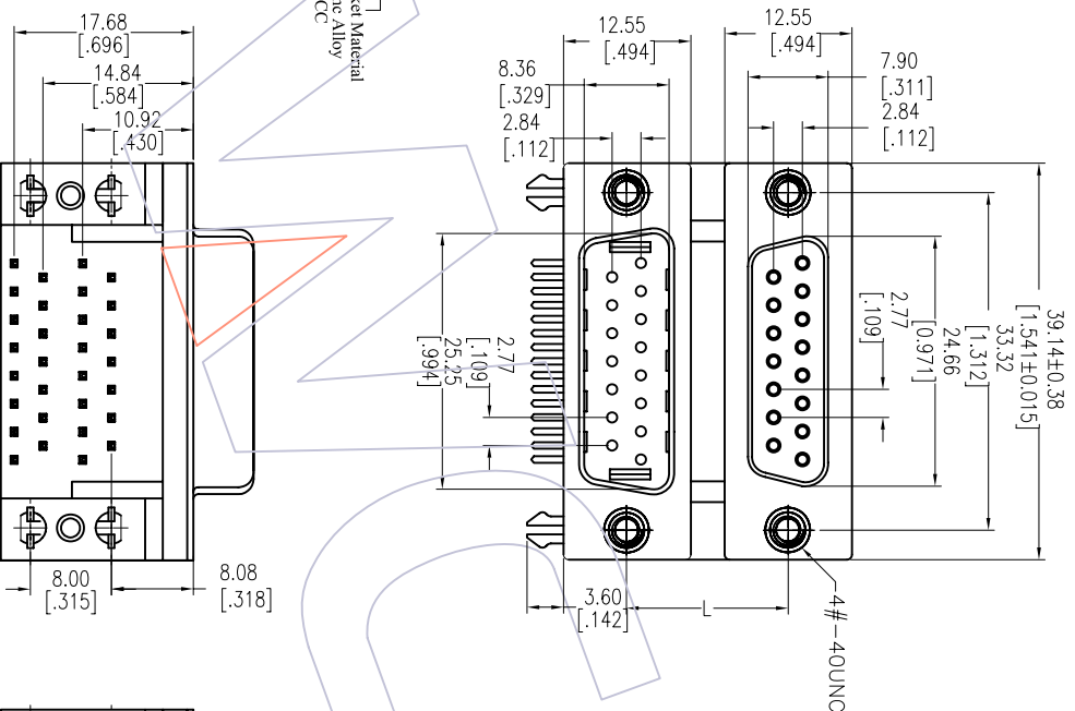
6200-X15FX15MXXX11(WITHOUT SCREW)
