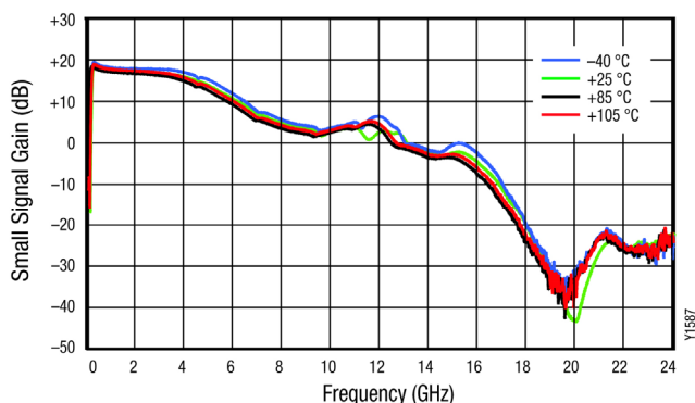
Figure 5. Broadband Gain vs Frequency over Temperature
