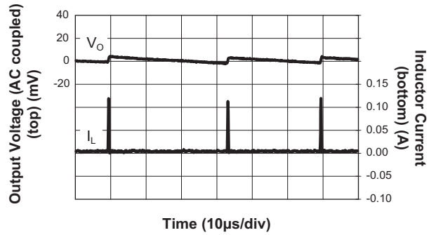
Output Ripple
