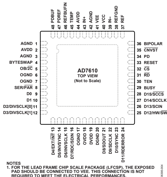
Figure 4. Pin Configuration
