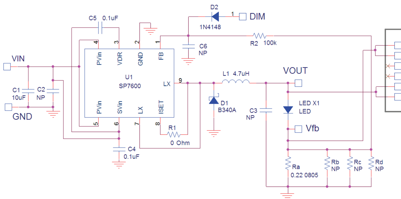
Figure 1. The SP7600 Evaluation Board Schematic Diagram
