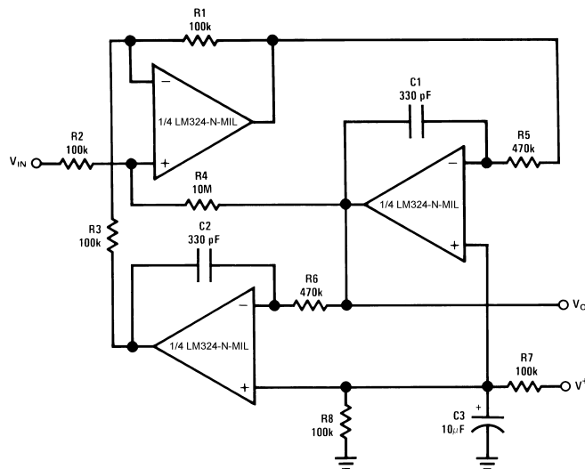
Figure 16. Power Amplifier
