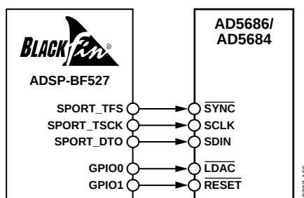
Figure 44. SPORT Interface
