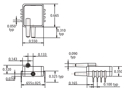
D4 Package
