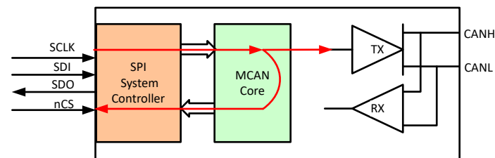
图 8-13. M_CAN External Loop Back Test Mode
