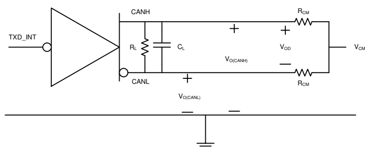
图 7-4. Driver Test Circuit and Measurement
