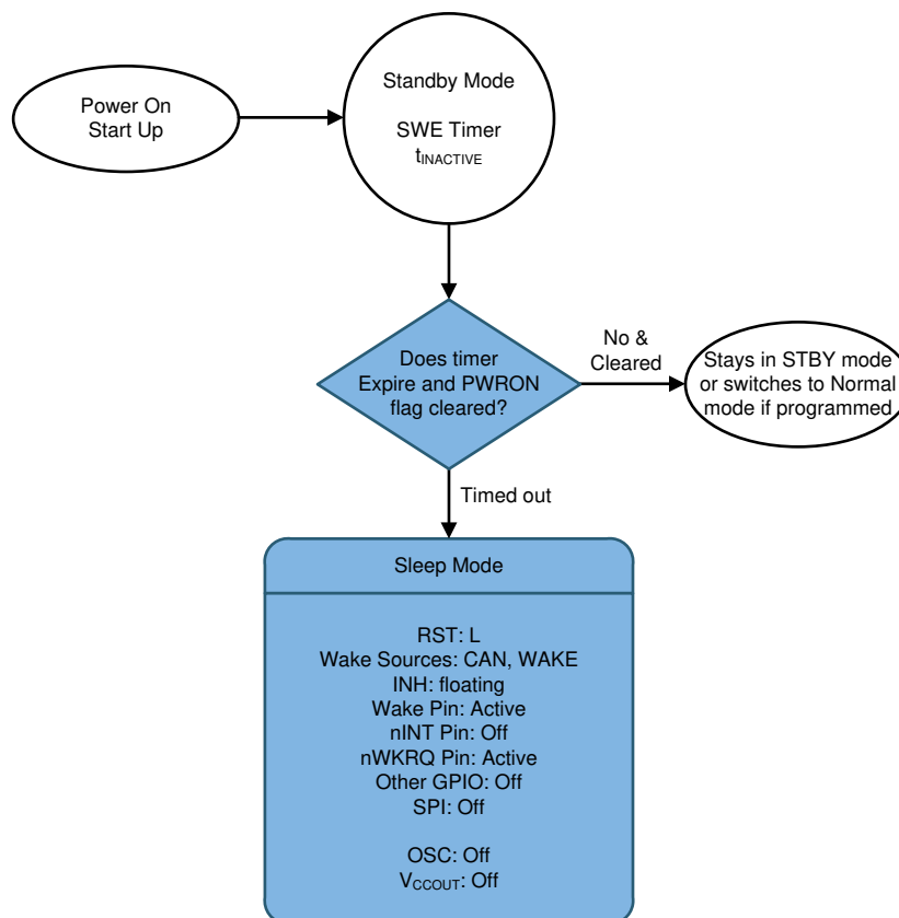
图 8-14. Power On Failsafe Feature
