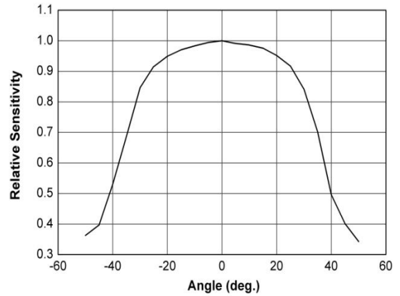
Fig.-5 Relative Sensitivity vs. Angle
