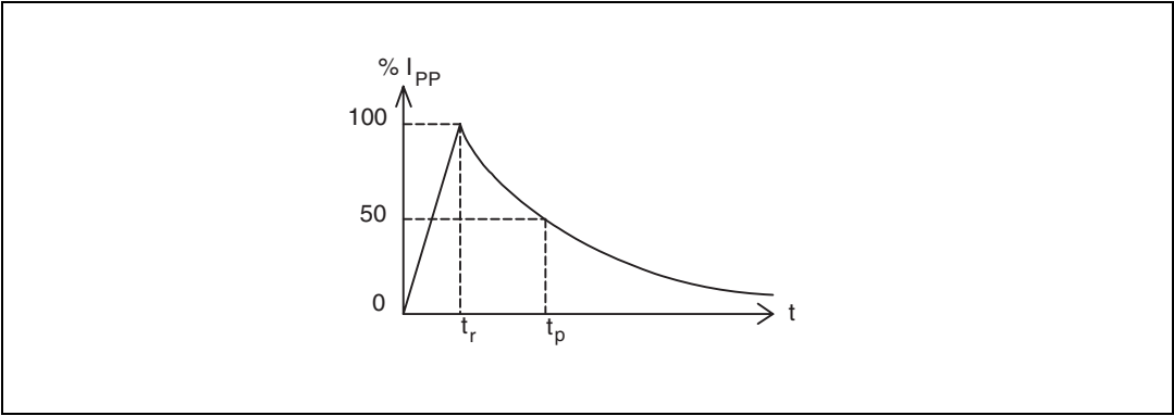
Figure 2. Pulse waveform 10/1000 \mu\text{s} , t_r = 10\text{ }\mu\text{s} , t_p = 1000\text{ }\mu\text{s}
