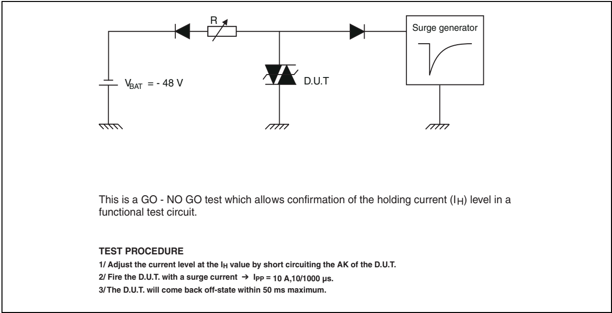
Figure 5. Test circuit 2 for I_H parameter
