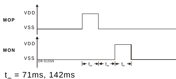
Figure 4: Motor drive on MON and MOP pins of device
