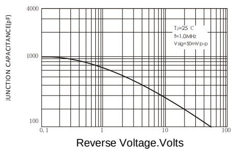
Typical Juncyion Capacitance
