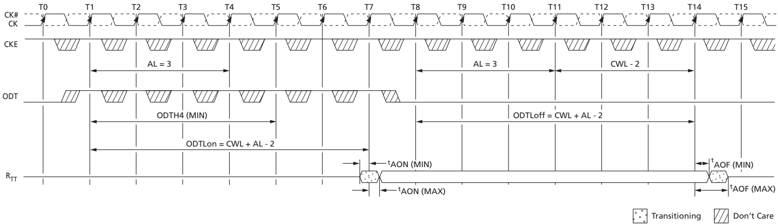
Figure 115: Synchronous ODT
