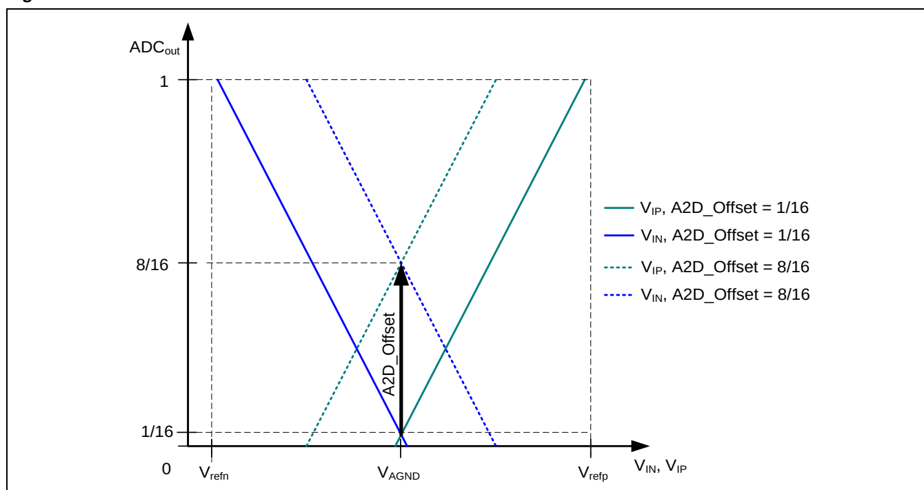
Figure 2.2 ADC Offset
