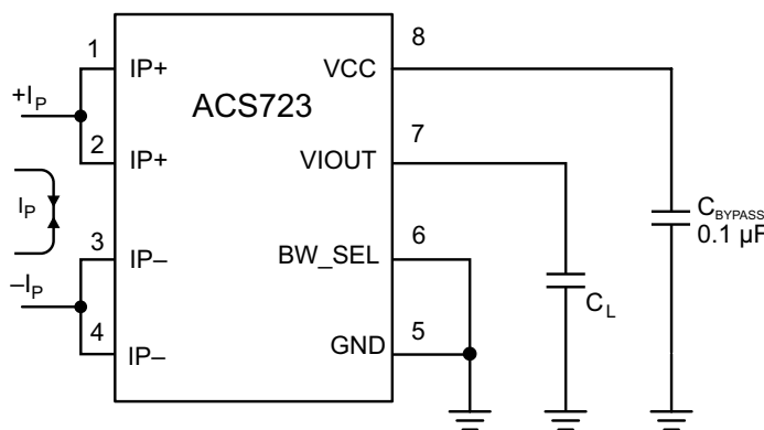
Typical Application
