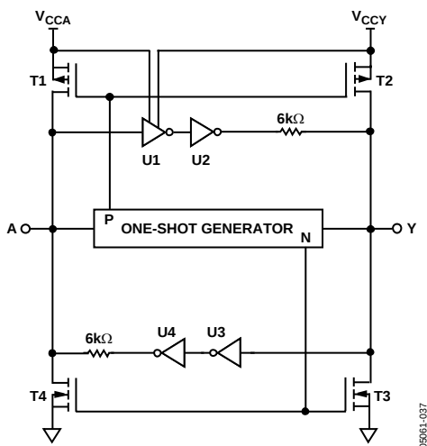
Figure 35. Simplified Block Diagram of an ADG3300 Channel
