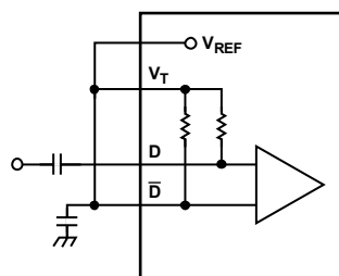
CONNECT V_T , V_{REF} , AND \bar{D} . PLACE A BYPASS CAPACITOR FROM V_T TO GROUND. ALTERNATIVELY, V_T , V_{REF} , AND D CAN BE CONNECTED, GIVING A CLEANER LAYOUT AND A 180^\circ PHASE SHIFT.
