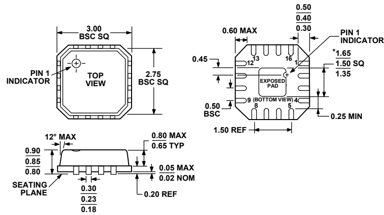
*COMPLIANT TO JEDEC STANDARDS MO-220-VEED-2 EXCEPT FOR EXPOSED PAD DIMENSION. Figure 31. 16-Lead Lead Frame Chip Scale Package [LFCSP_VQ] 3 mm × 3 mm Body, Very Thin Quad (CP-16-3) Dimensions shown in millimeters
