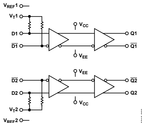
Figure 2. ADCLK907 ECL Dual 1:1 Clock/Data Buffer
