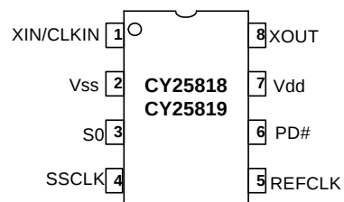
8-pin SOIC
