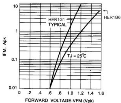
Fig. 2 - FORWARD CHARACTERISTICS
