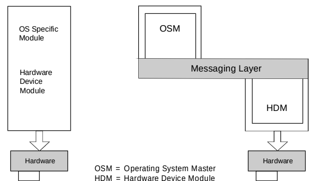
Figure 3-13. I 2 O Software Architecture
