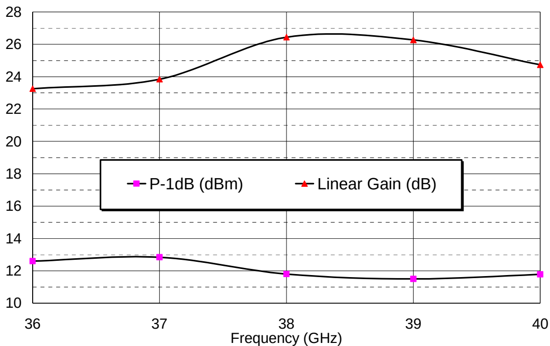
Linear Gain &amp; Output power @ 1dB compression versus frequency
