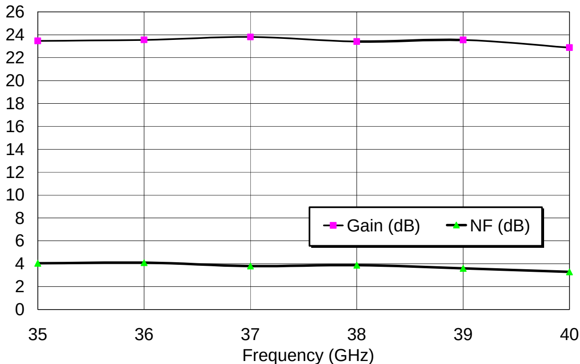
Gain &amp; Noise Figure versus frequency
