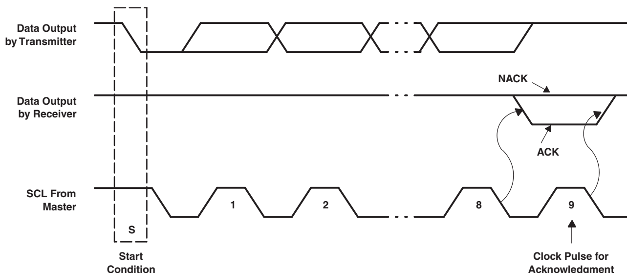
Figure 12. Acknowledge on I 2 C Bus
