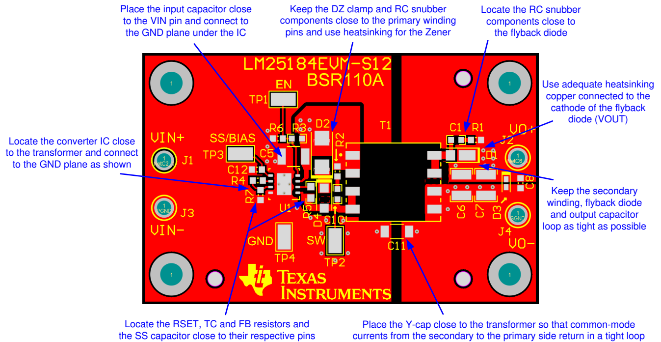
Figure 47. Single-Output PCB Layout Example
