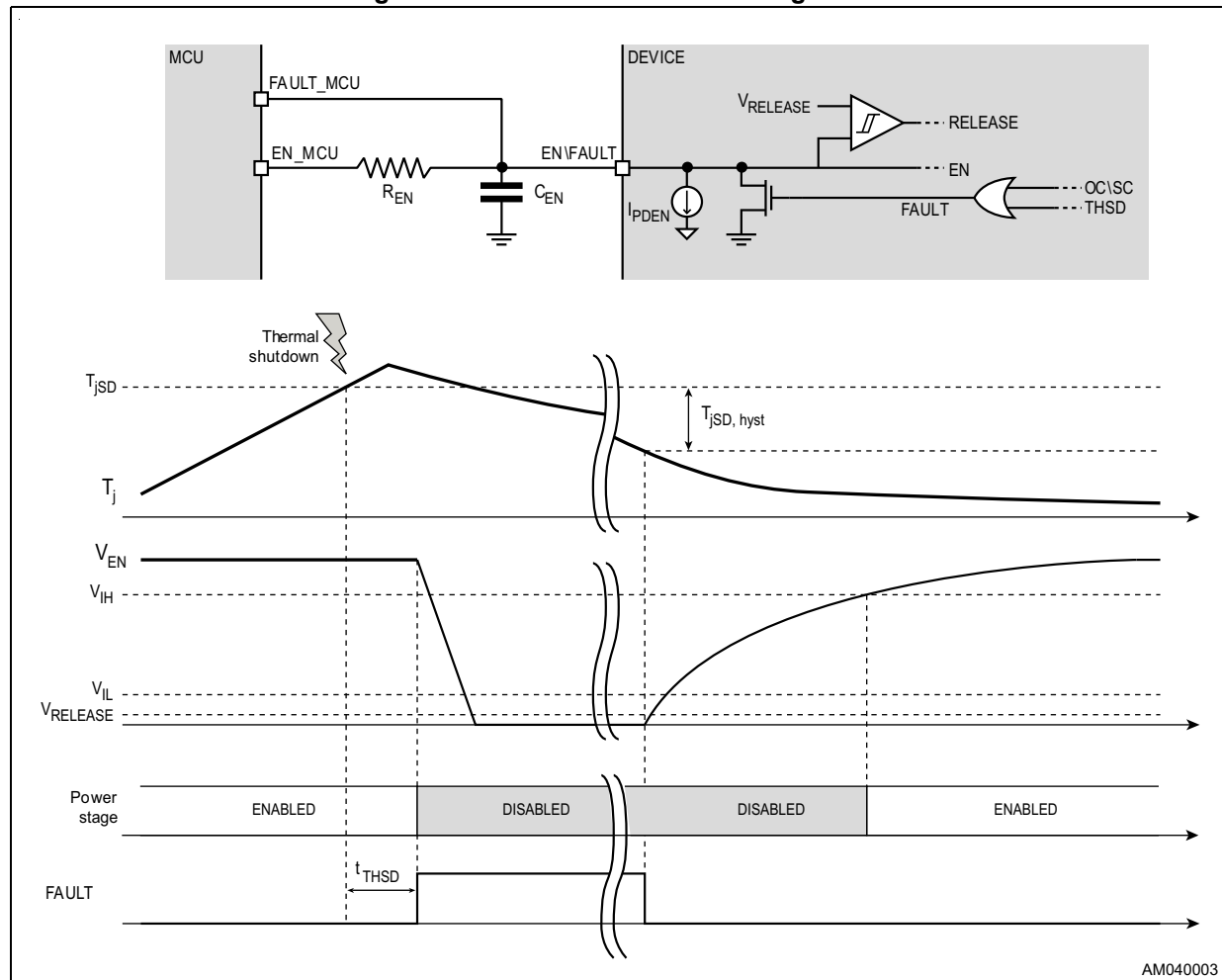
Figure 11. Thermal shutdown management
