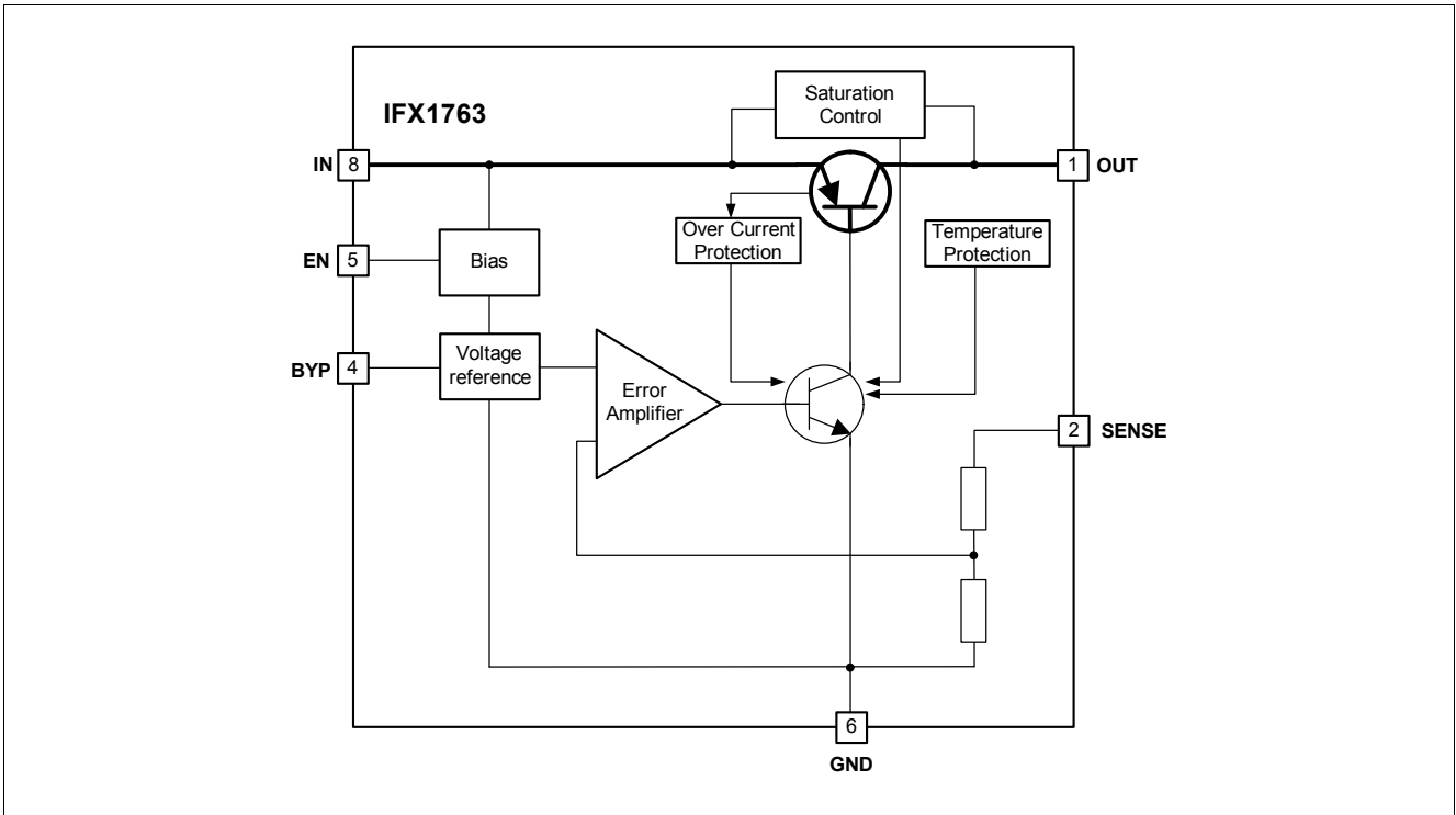
Figure 1 Block Diagram IFX1763 fixed voltage version
