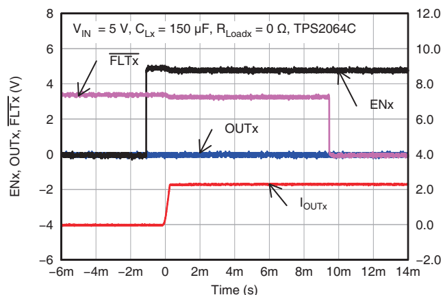
Figure 23. TPS2064C Enable into Short
