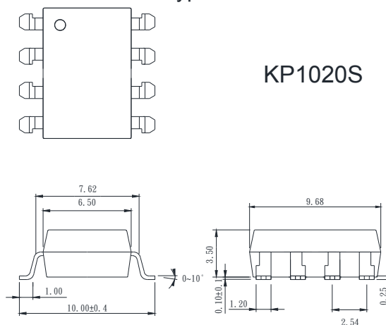
2. Surface mount type.
