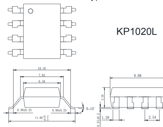
4. Long creepage distance for surface mount type.
