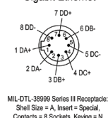
Gigabit Ethernet
