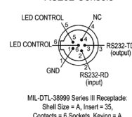
RS232 Console
