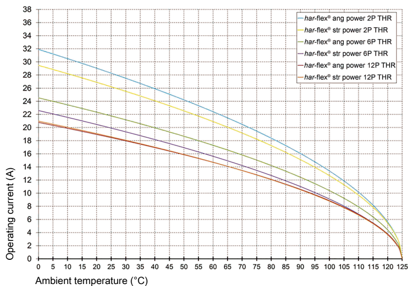
Derating curve 80%
