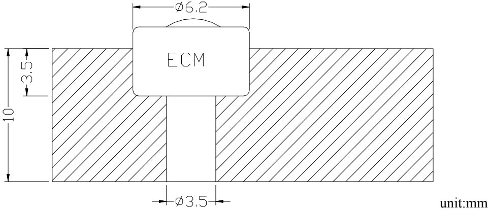
7-8 固定部孔形状 Shape of hole at fixed part
