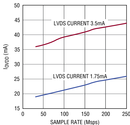
LTC2152-12: I_{OVPD} vs Sample Rate, 15MHz Sine Wave Input, -1\text{dBFS}
