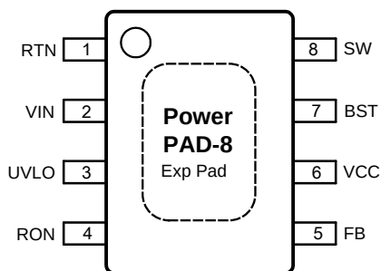
Figure 1. Top View
