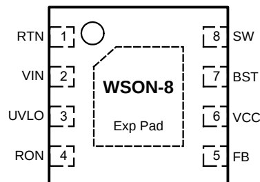
Figure 2. Top View
