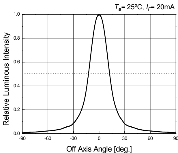
Directivity
