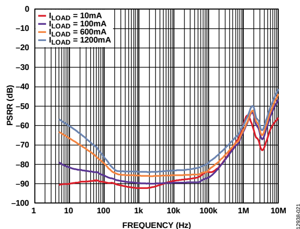
Figure 21. Power Supply Rejection Ratio (PSRR) vs. Frequency at Various Loads, V_{OUT} = 3.3\text{ V}
