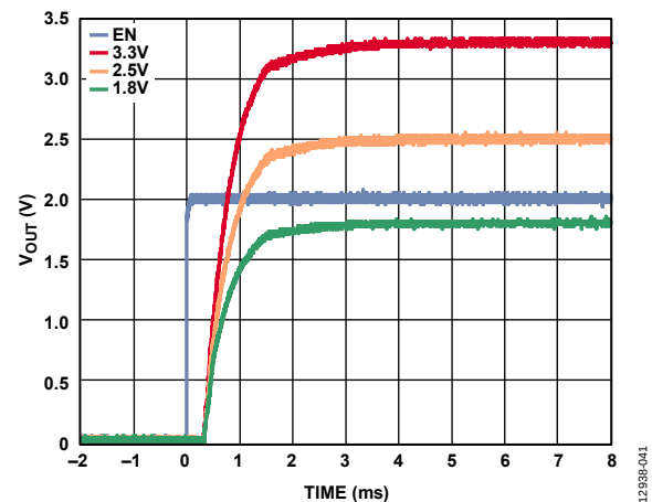
Figure 39. V_{OUT} Start-Up Time After V_{EN} Rising at Various Output Voltages, V_{IN} = 5.0 \text{ V} , C_{BYP} = 1 \mu\text{F}
