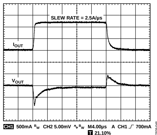
Figure 44. Output Transient Response, V_{\text{OUT}} = 3.3\text{ V} , C_{\text{OUT}} = 10\text{ }\mu\text{F} , Channel 1 = Load Current, Channel 2 = V_{\text{OUT}}
