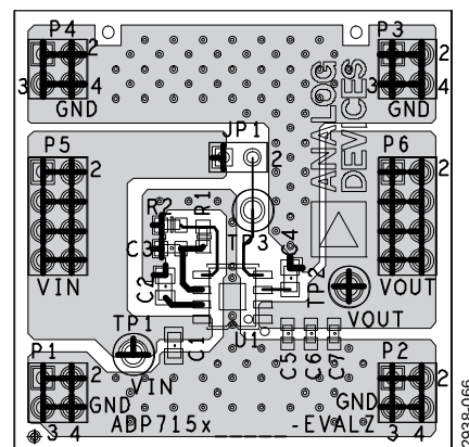
Figure 64. Sample 8-Lead SOIC PCB Layout
