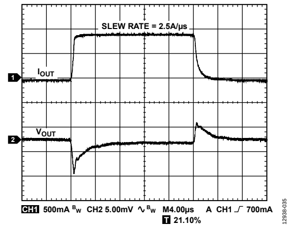
Figure 33. Load Transient Response, I_{LOAD} = 100 \text{ mA} to 1.2 \text{ A} , V_{OUT} = 3.3 \text{ V} , V_{IN} = 4.0 \text{ V} , Channel 1 = I_{OUT} , Channel 2 = V_{OUT}
