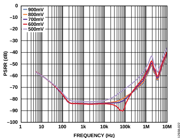
Figure 22. Power Supply Rejection Ratio (PSRR) vs. Frequency at Various Headroom Voltages, V_{OUT} = 3.3\text{ V} , 1.2\text{ A Load}
