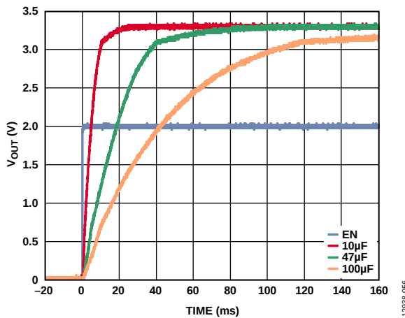
Figure 54. Typical Start-Up Behavior with C_{BYP} = 1 \mu F to 100 \mu F
