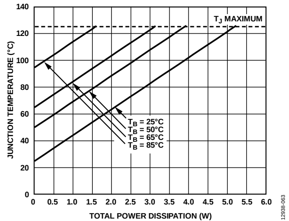
Figure 61. Junction Temperature vs. Total Power Dissipation for the 10-Lead LFCSP
