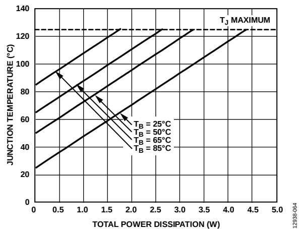
Figure 62. Junction Temperature vs. Total Power Dissipation for the 8-Lead SOIC
