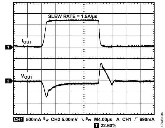
Figure 34. Load Transient Response, I_{LOAD} = 100 \text{ mA} to 1.2 \text{ A} , V_{OUT} = 3.3 \text{ V} , V_{IN} = 4.0 \text{ V} , C_{OUT} = 22 \mu\text{F} , Channel 1 = I_{OUT} , Channel 2 = V_{OUT}
