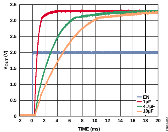
Figure 53. Typical Start-Up Behavior with C_{BYP} = 1 \mu F
