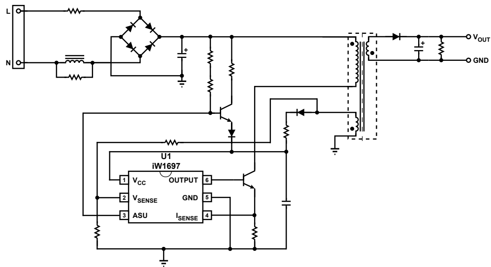
Figure 3.2: iW1697 Typical Application Circuit (Achieving < 20 mW No-load Power Consumption. Using NPN BJT as Active Start-up Device)
