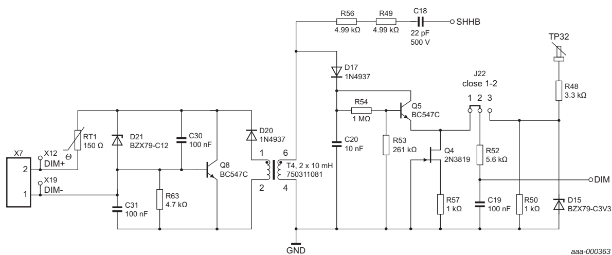
Fig 14. Schematic diagram: dim input circuit
