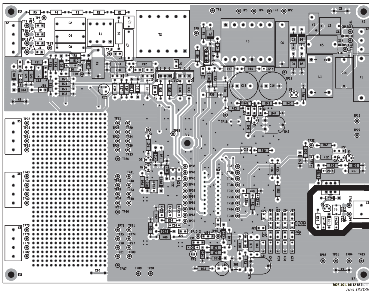
Fig 17. Evaluation board (bottom view)
