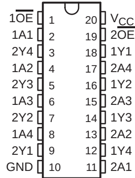
SN54LVT244 . . . J OR W PACKAGE SN74LVT244 . . . DB, DW, OR PW PACKAGE (TOP VIEW)
